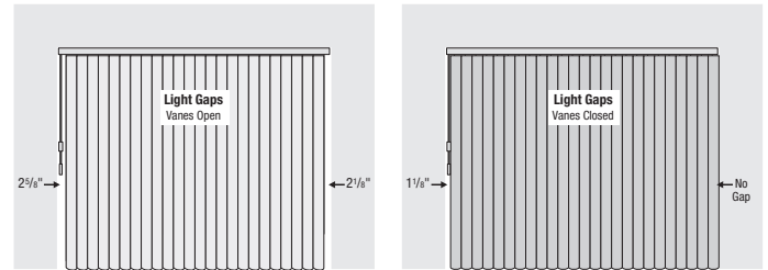
Figure 2: Light gaps occur with IB applications.
