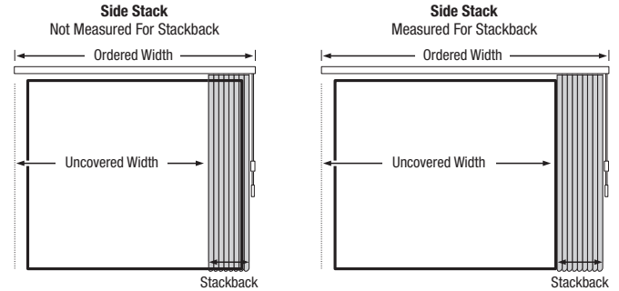
Figure 1: Measuring for side stack with and without stackback.
